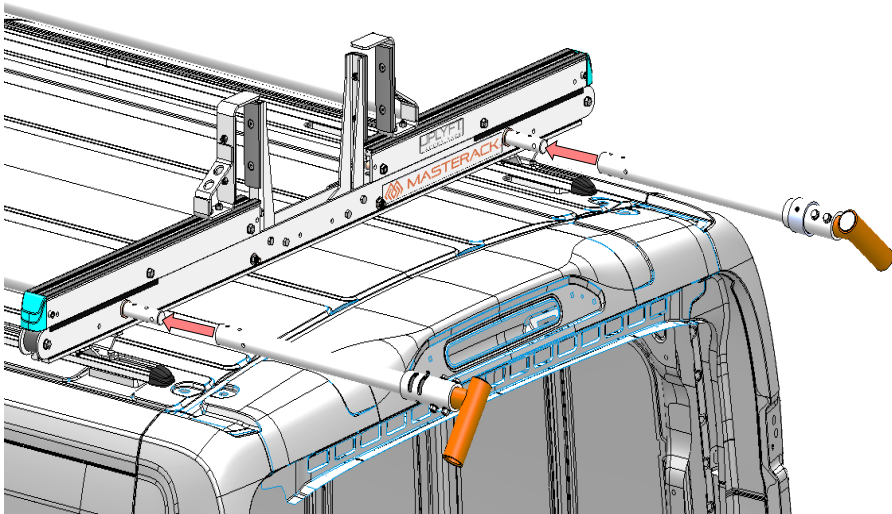
Step 14. Install handle assembly into rear crossbow
