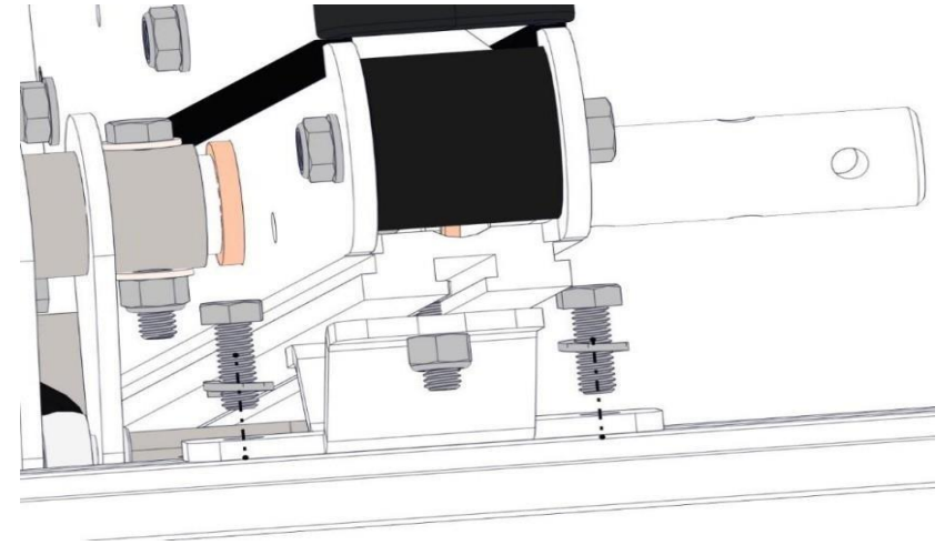
Step 9. Install 5/16 X 7/8 bolts (4) with lock washers (4) through crossbow mounts into receiver blocks and apply seize to bolts Do not tighten
