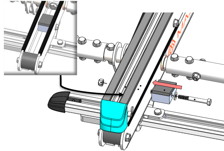
Step 17. Install ladder stops (2) on curbside crossbows using 5/16" x 2-1/2" bolts, washer, bumper stop and nut and tighten with a 1/2" wrench
