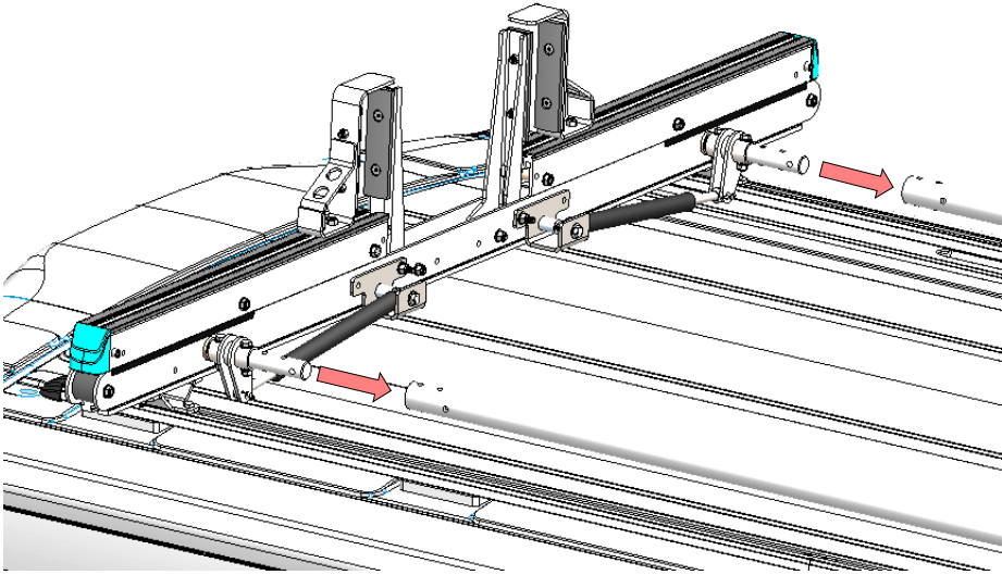
Step 12. Slide the rear crossbow into connecting tubes.
