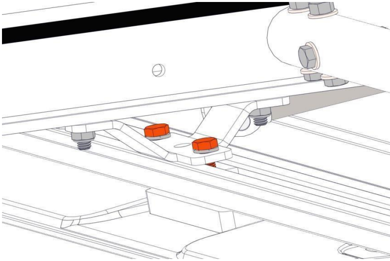
Step 16. Tighten crossbow bolts
