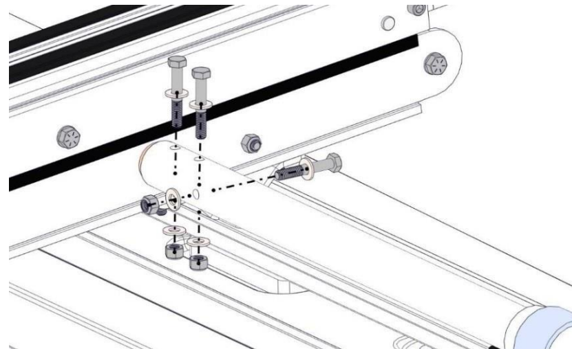
Step 15. Fasten handle with 5/16 X 2-1/2 bolts (6) and washers (12) and apply seize to bolts
