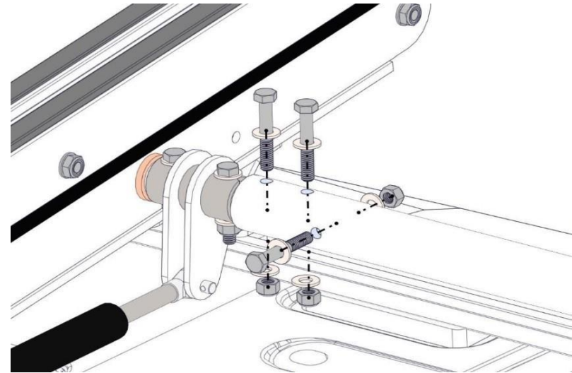
Step 11. Install connecting tubes with 5/16" X 2 - 1/2" fasteners (6) & washers (12) and apply seize to bolts.
