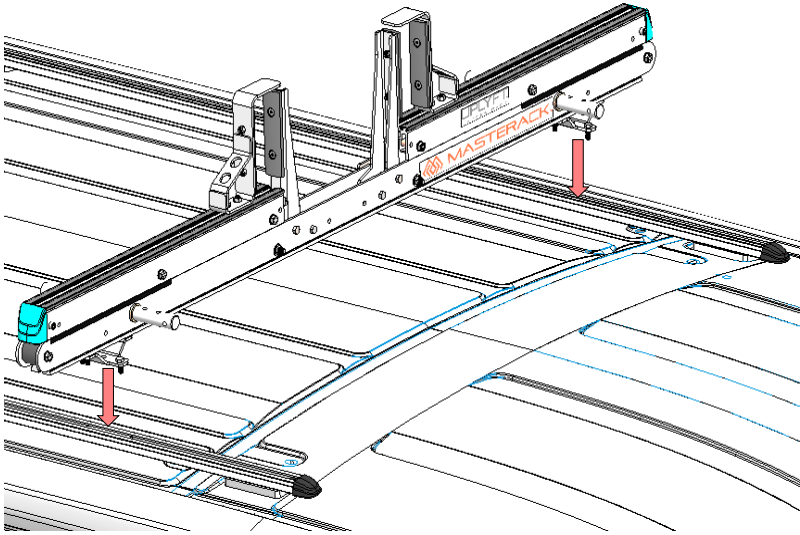
Step 8. Lay front crossbow across mounting rails.
