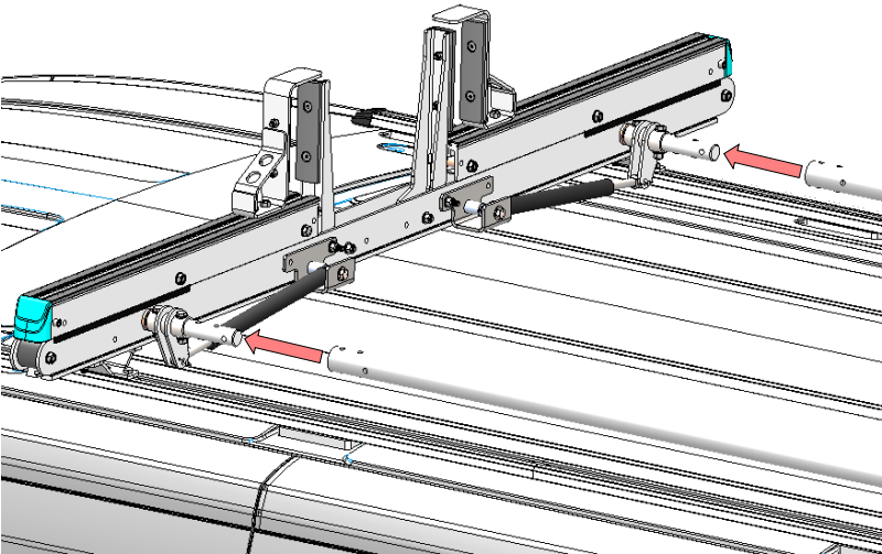
Step 10. Slide Connecting tubes (02P328) into front crossbow. Line holes up with crossbow rod and connecting tube.
